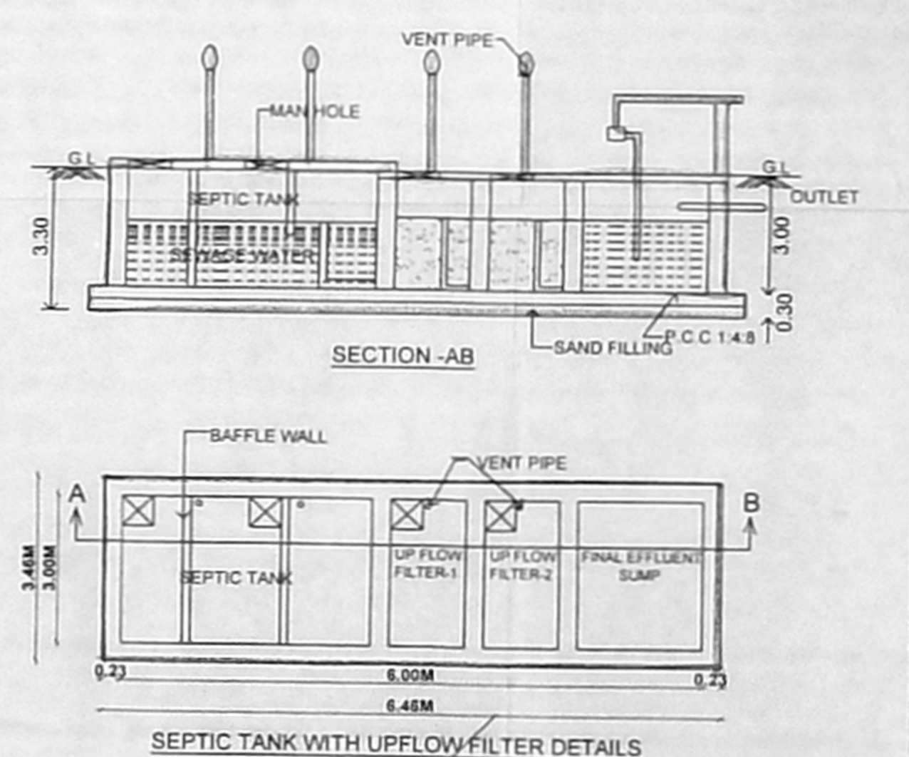
SEPTIC TANK WITH UPFLOW FILTER DETAILS
