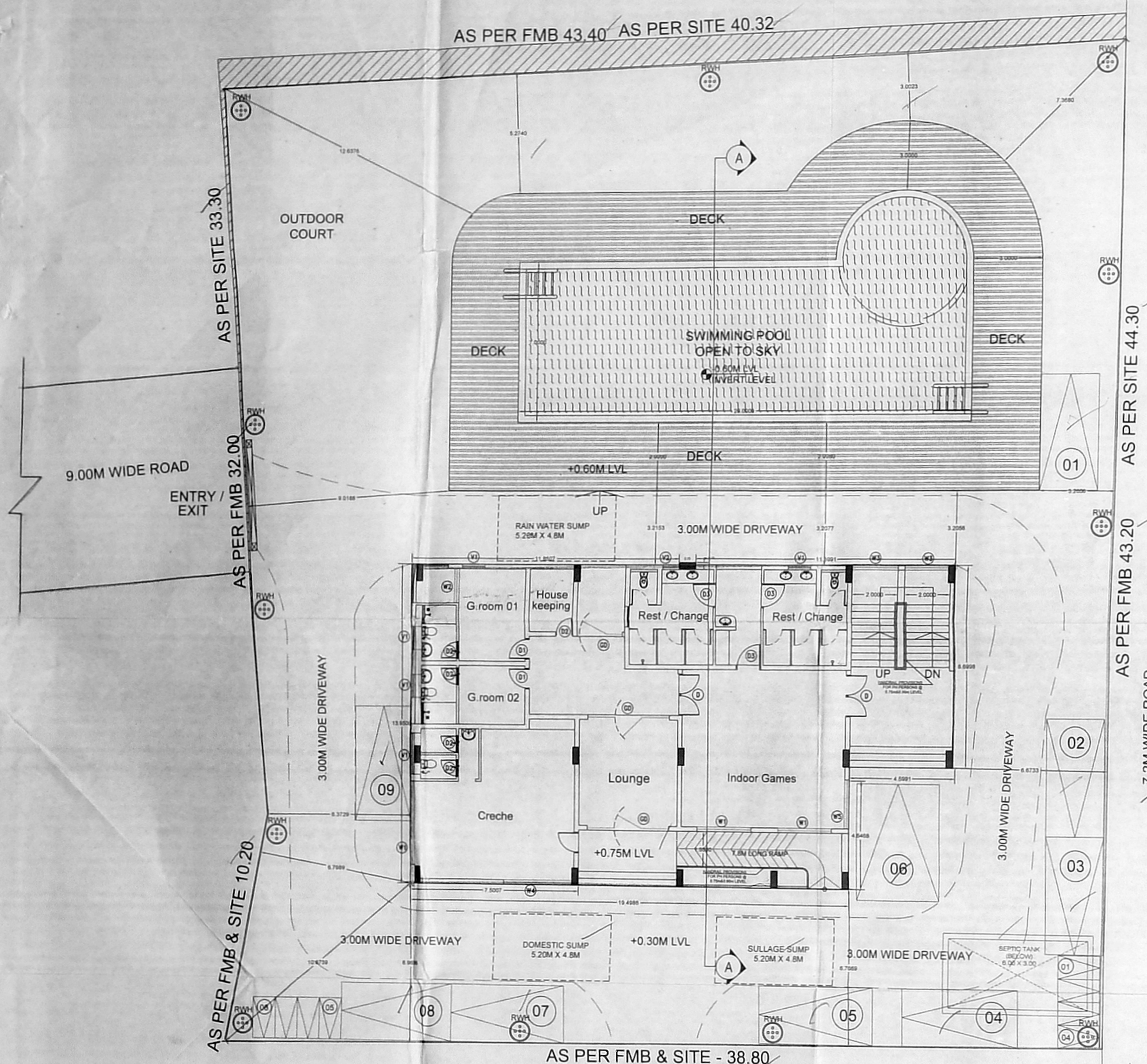
SITE CUM GROUND FLOOR & SWIMMING POOL PLAN
